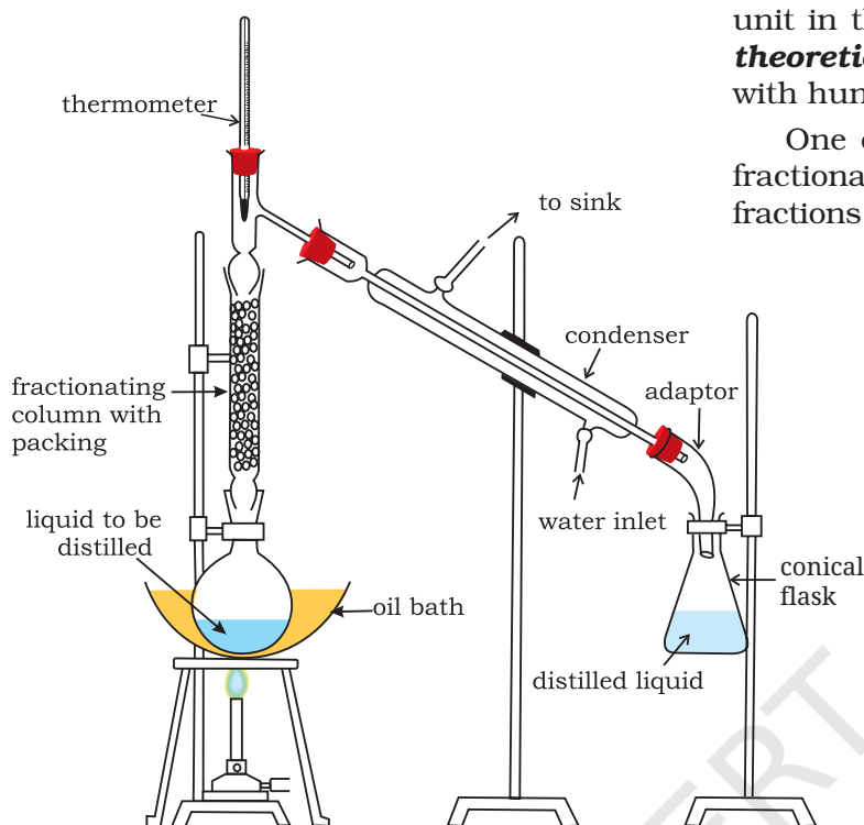
Fig.8.6 Fractional distillation. The vapours of lower boiling fraction reach the top of the column first followed by vapours of higher boiling fractions.
