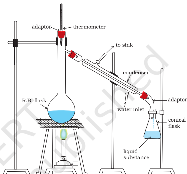
Fig.8.5 Simple distillation. The vapours of a substance formed are condensed and the liquid is collected in conical flask.
