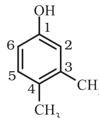
3,4-Dimethylphenol
